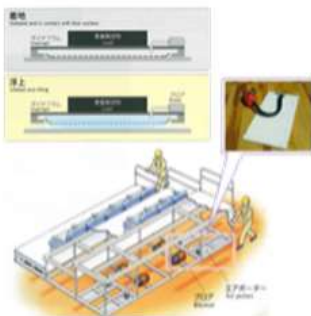
Heavy Load Transport System Air Bearing/ Air Porter
